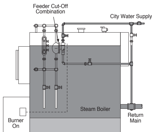
Large Boilers
